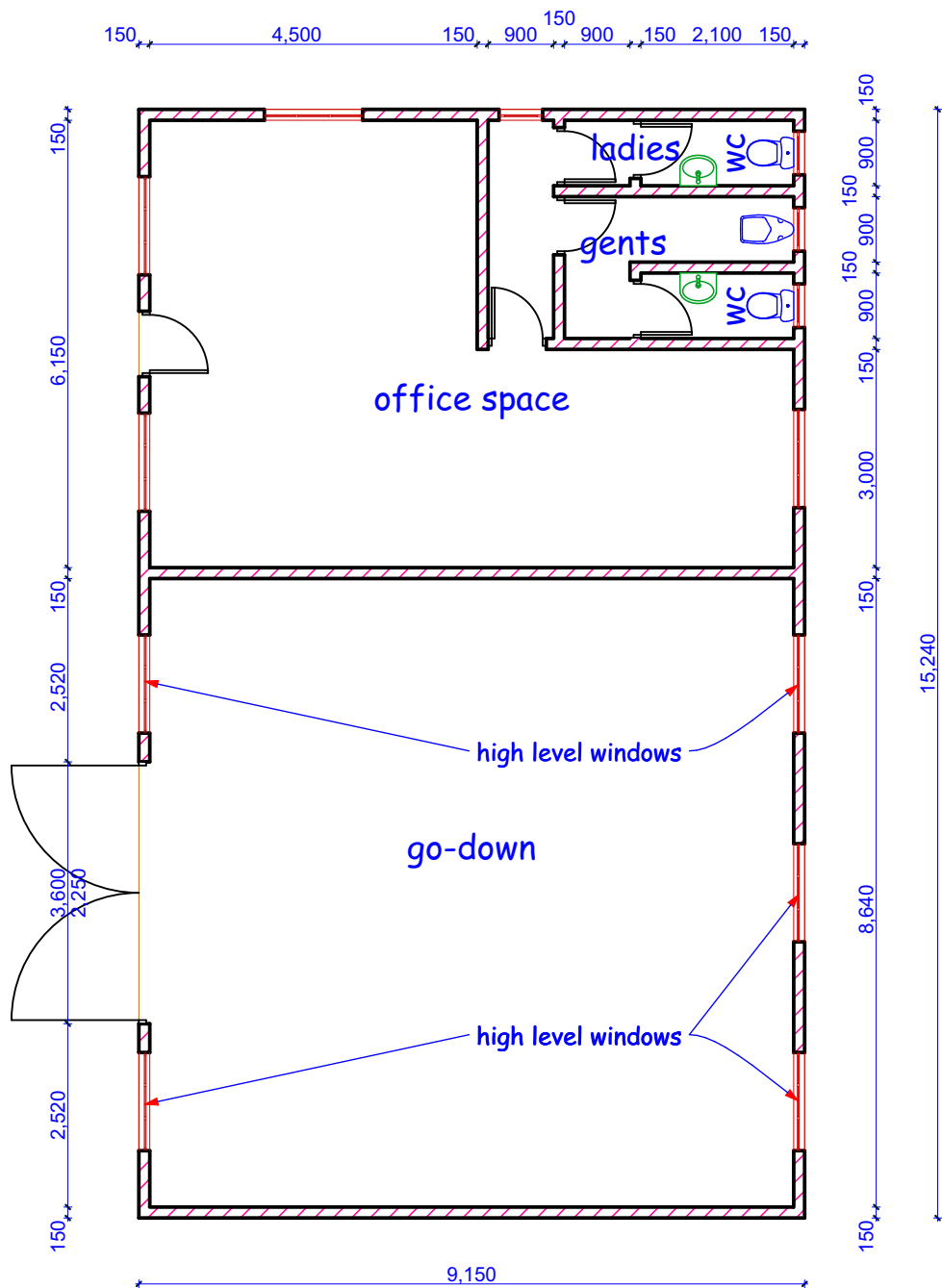
floor plan 1:100
